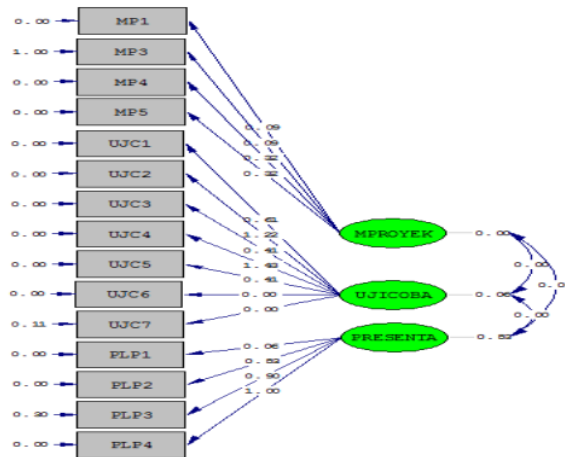
Figure 4. Confirmatory Factor Analysis Model Syntax
